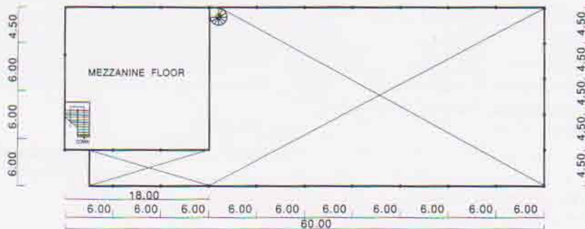
MEZZANINE FLOOR PLAN
