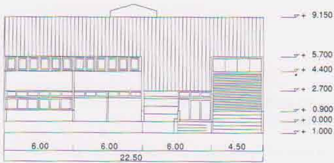
FRONT ELEVATION ( 1 UNIT )
